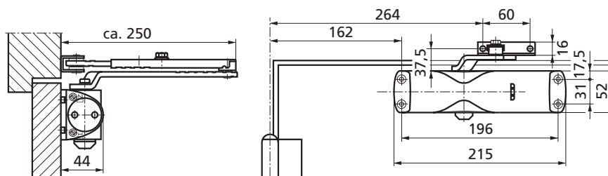
Dimensions EN size 4 max. opening angle approx. 110°
