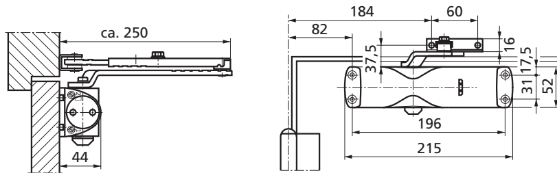
Dimensions EN size 4 max. opening angle approx. 110°
